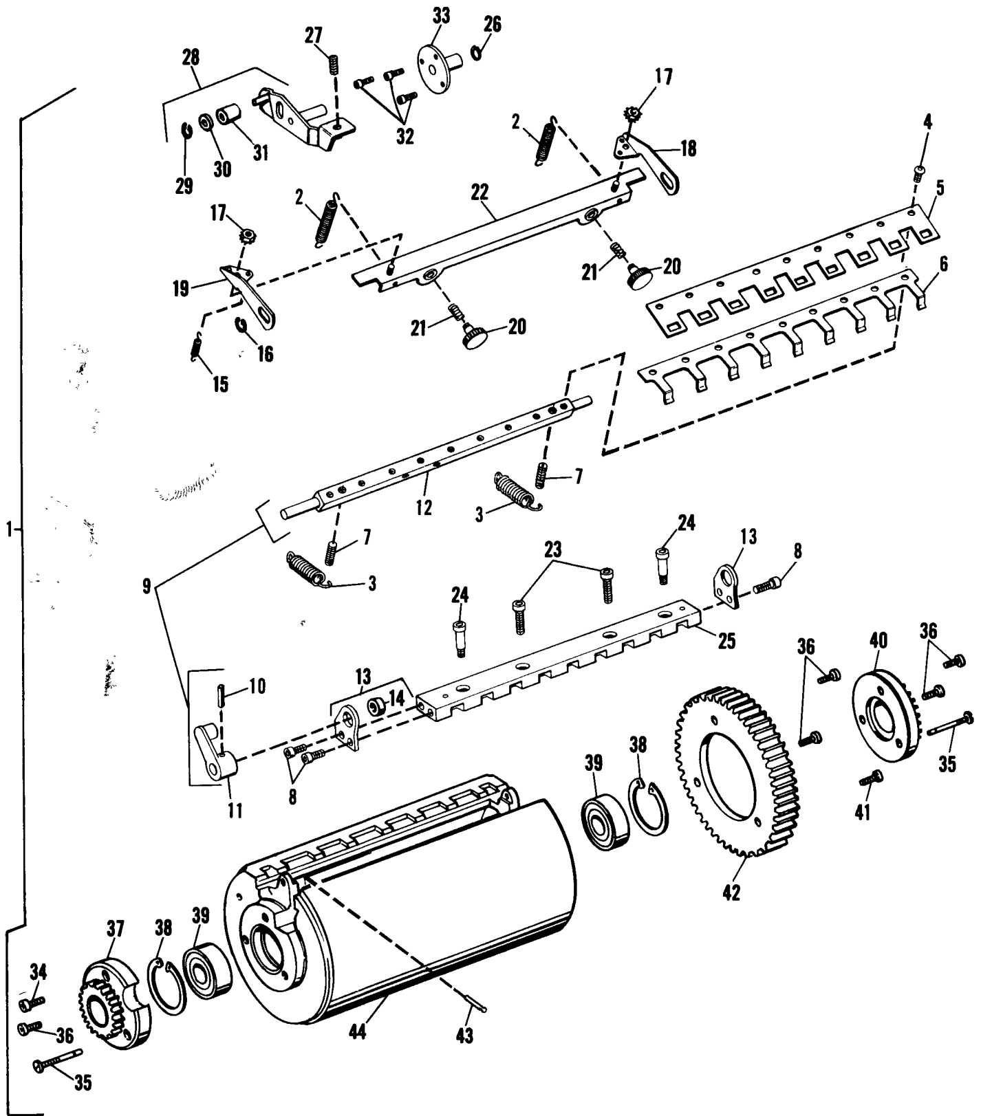
FIGURE 31 - MODEL 9865/9869 Master Cylinder Assembly
