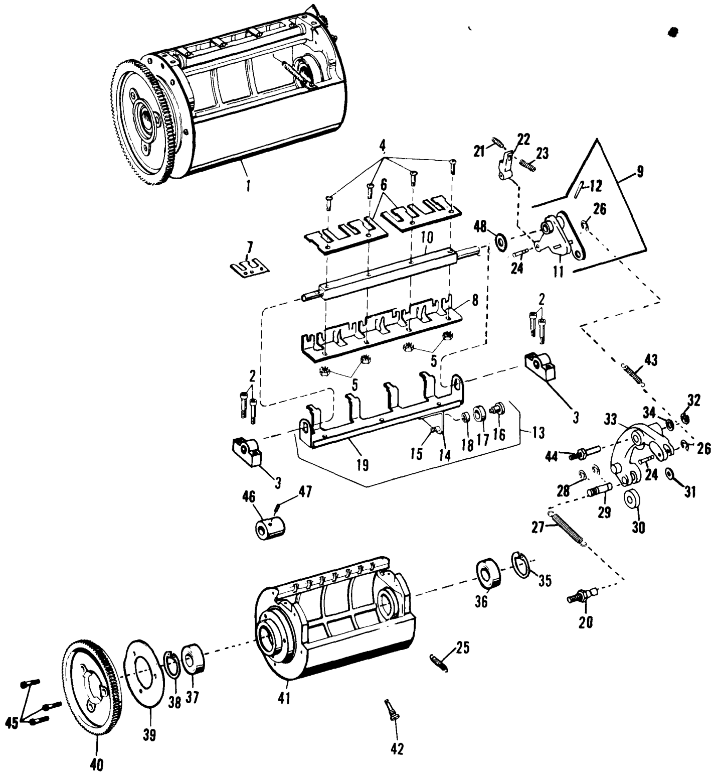
FIGURE 47 - MODEL 9865/9869 Impression Cylinder Assembly
