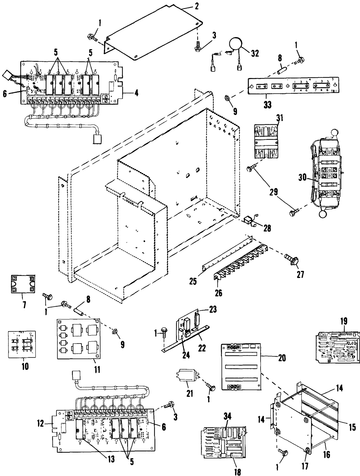
FIGURE 75 - MODEL 9865/9869 Control Box P.C.Boards
