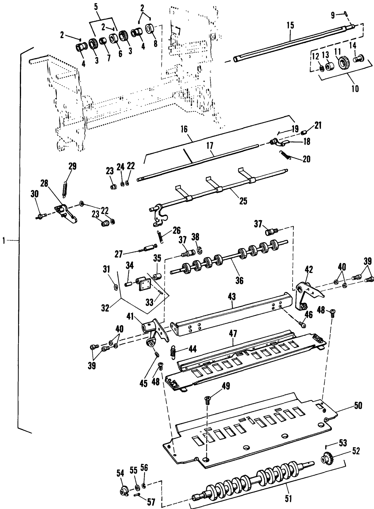
FIGURE 28 - MODEL 9865/9869 Master Forwarding Unit - Part I
