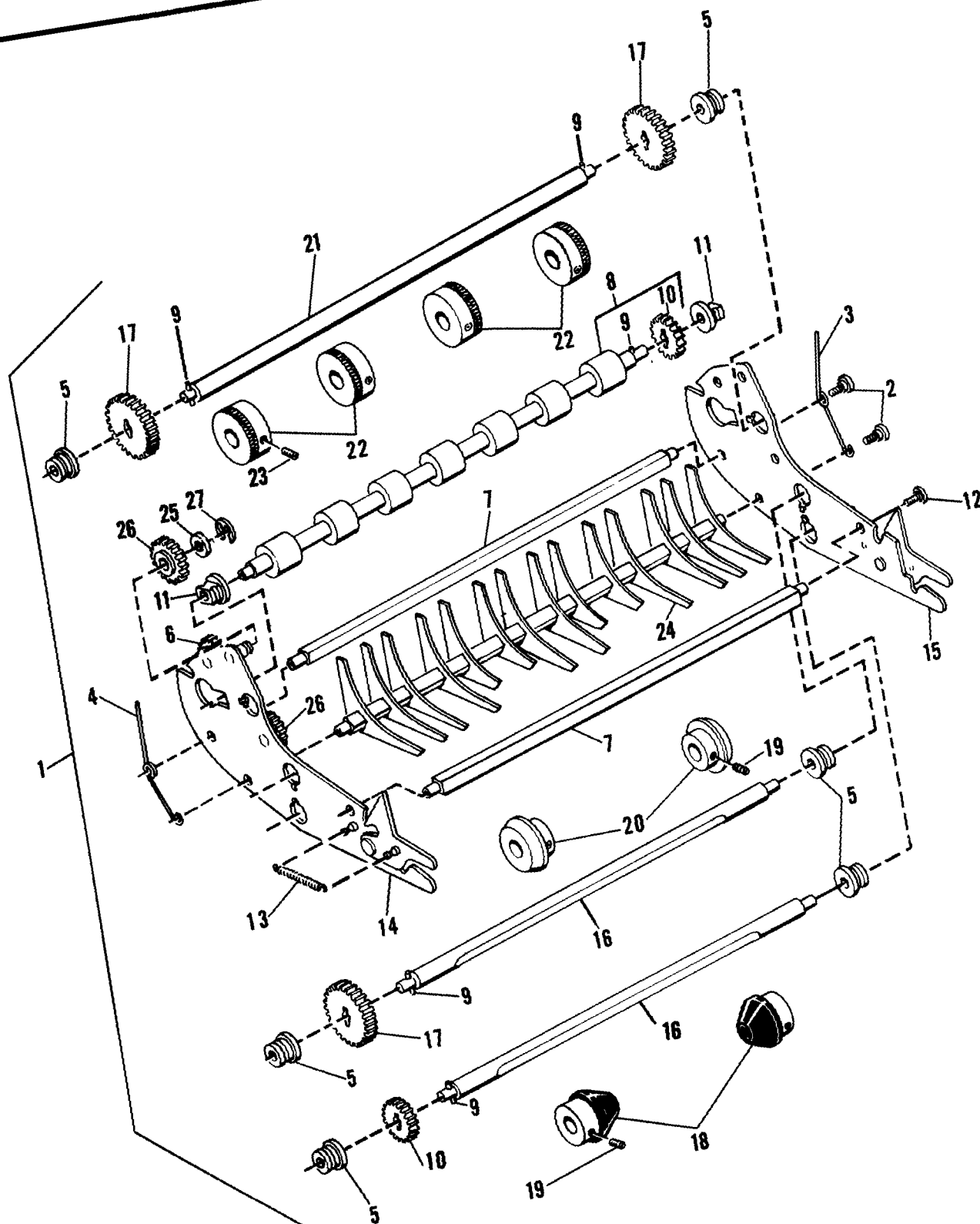
FIGURE 33 - MODEL 9865/9869 Master Ejector Assembly
