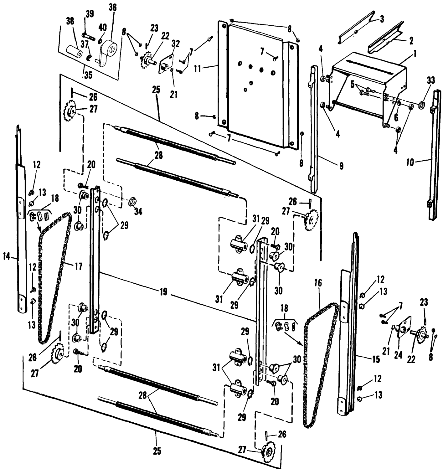
FIGURE 66 - MODEL 9865/9869 Feed Table and Paper Guides
