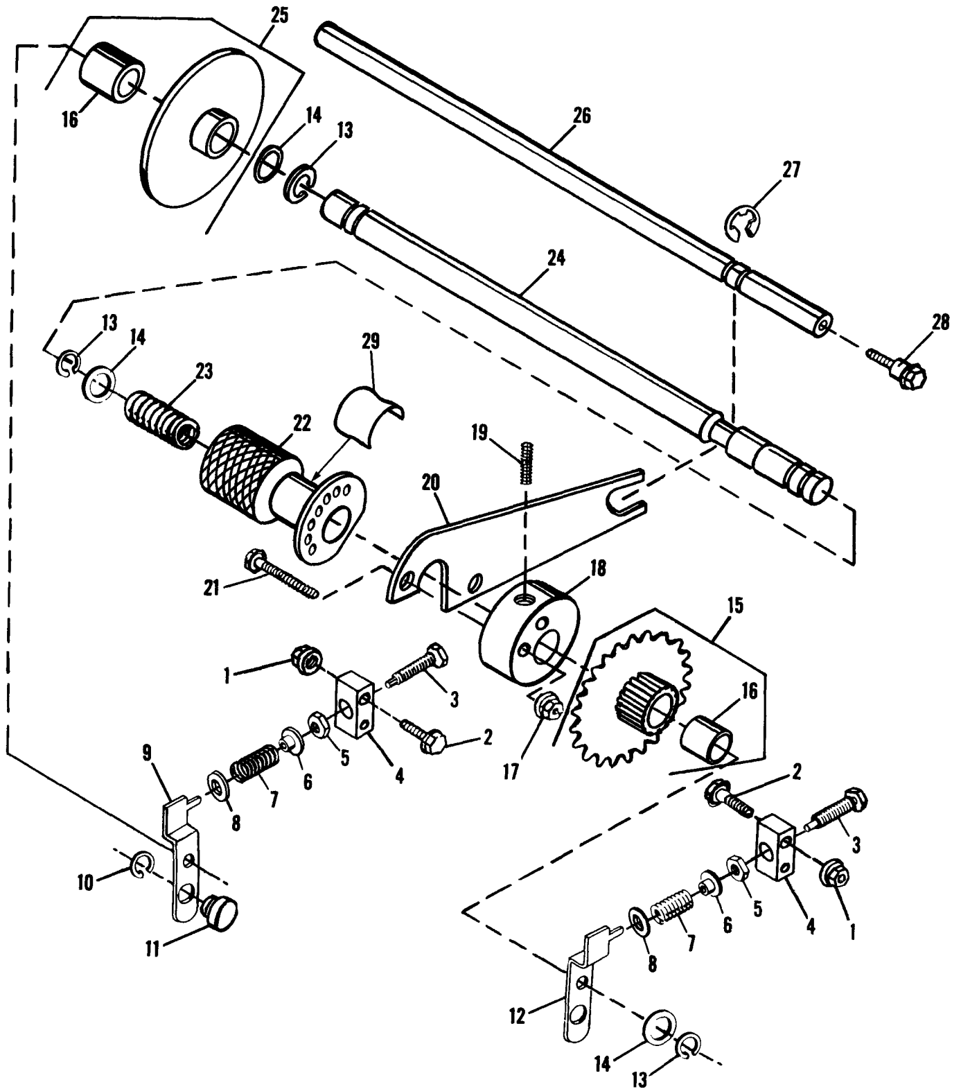
FIGURE 81 - MODEL 9865/9869 Idler Shaft Assembly
