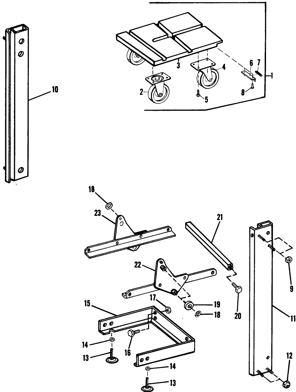
FIGURE 90 - MODEL 9865/9869 Dolly and Frame Assemblies
