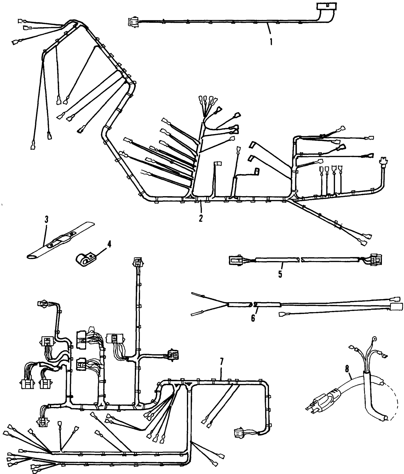
FIGURE 76 - MODEL 9865/9869 Control Box Harnesses - Part I
