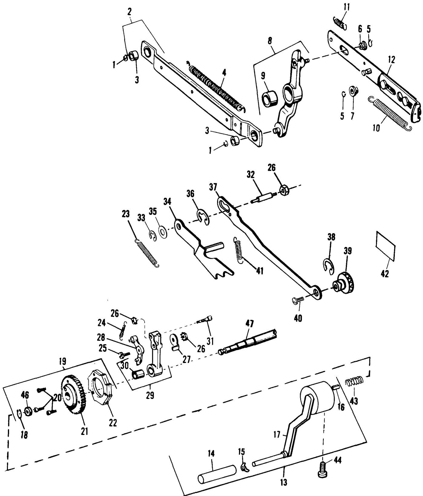
FIGURE 56 - MODEL 9865/9869 Feed Mechanism and Power Link
