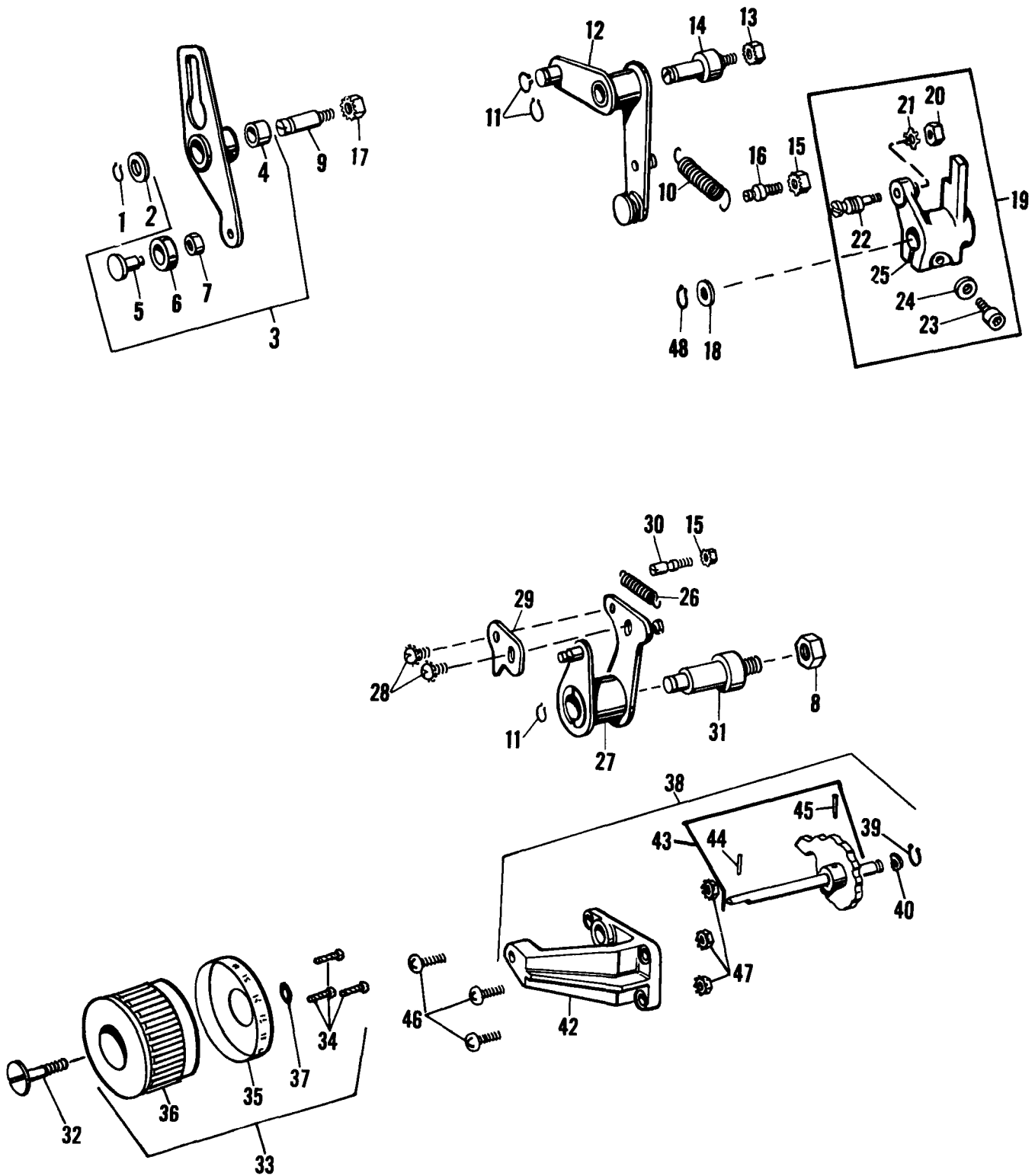
FIGURE 54 - MODEL 9865/9869 Buckle Adjusting and Lever Assemblies
