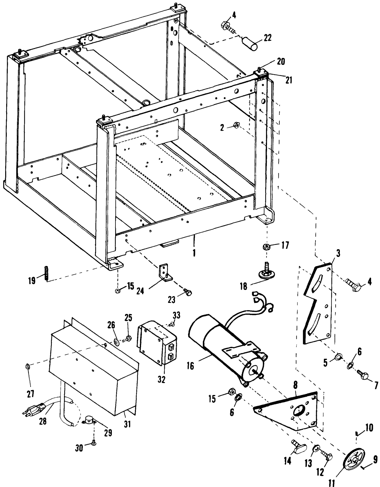
FIGURE 65 - MODEL 9865/9869 Base Frame and Drive Motor
