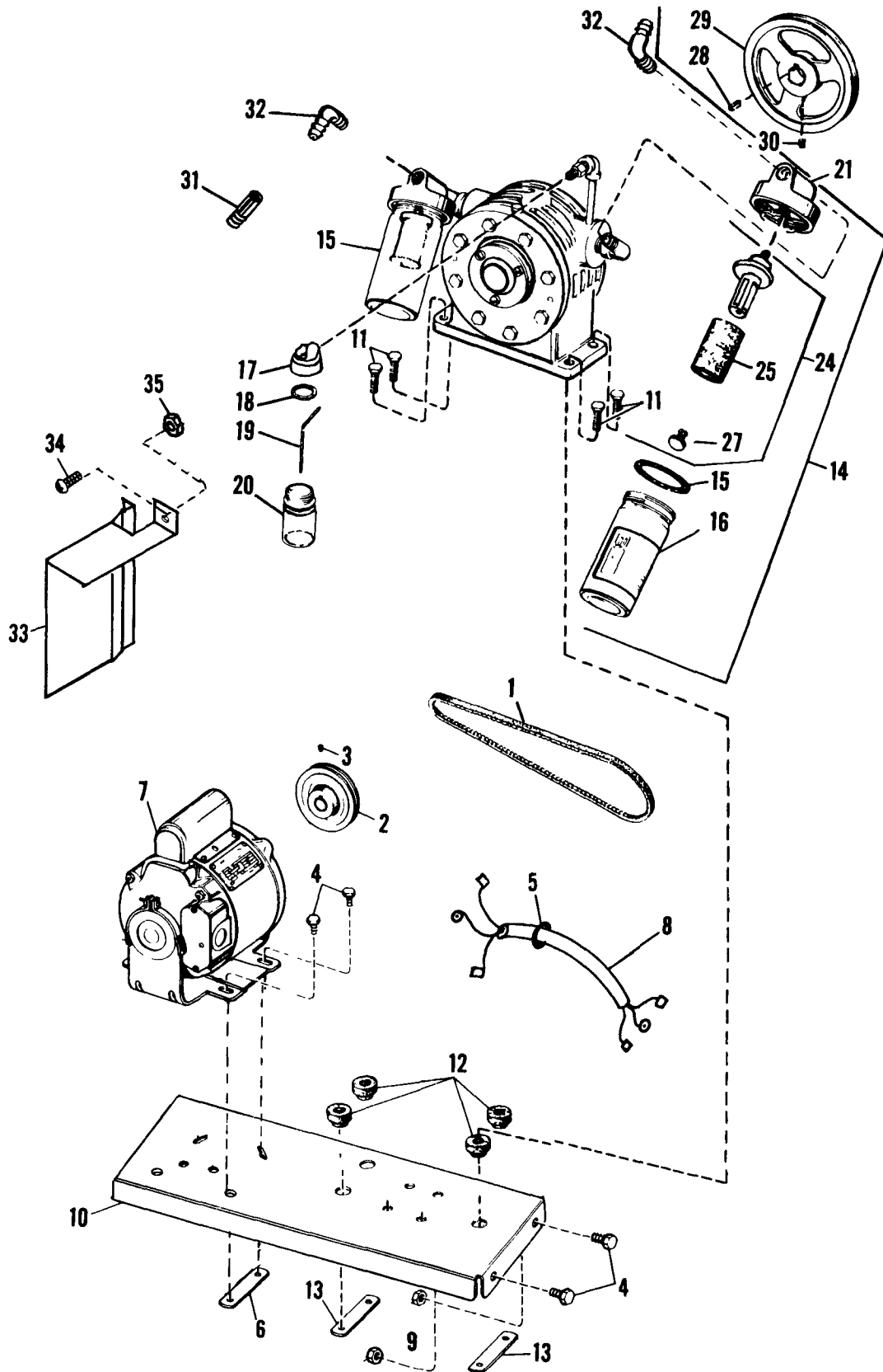
FIGURE 69 - MODEL 9865/9869 Compressor Assembly
