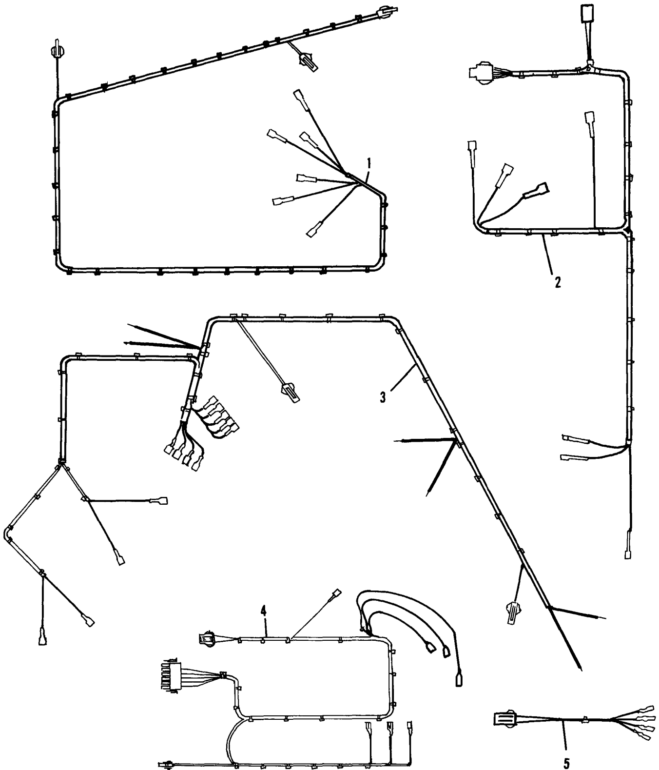
FIGURE 77 - MODEL 9865/9869 Control Box Harnesses - Part II
