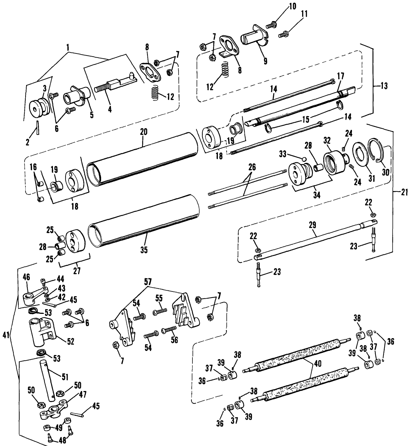
FIGURE 13 - MODEL 9865/9869 Waver, Oscillating and Rider Rollers
