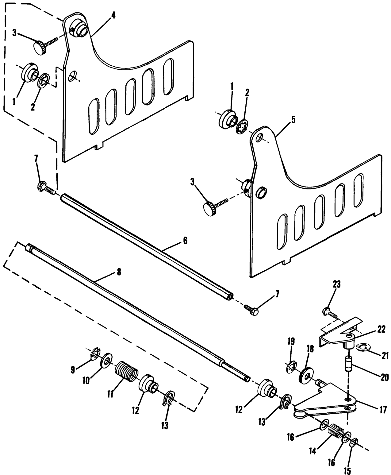
FIGURE 86 - MODEL 9865/9869 Paper Guides Chain Delivery
