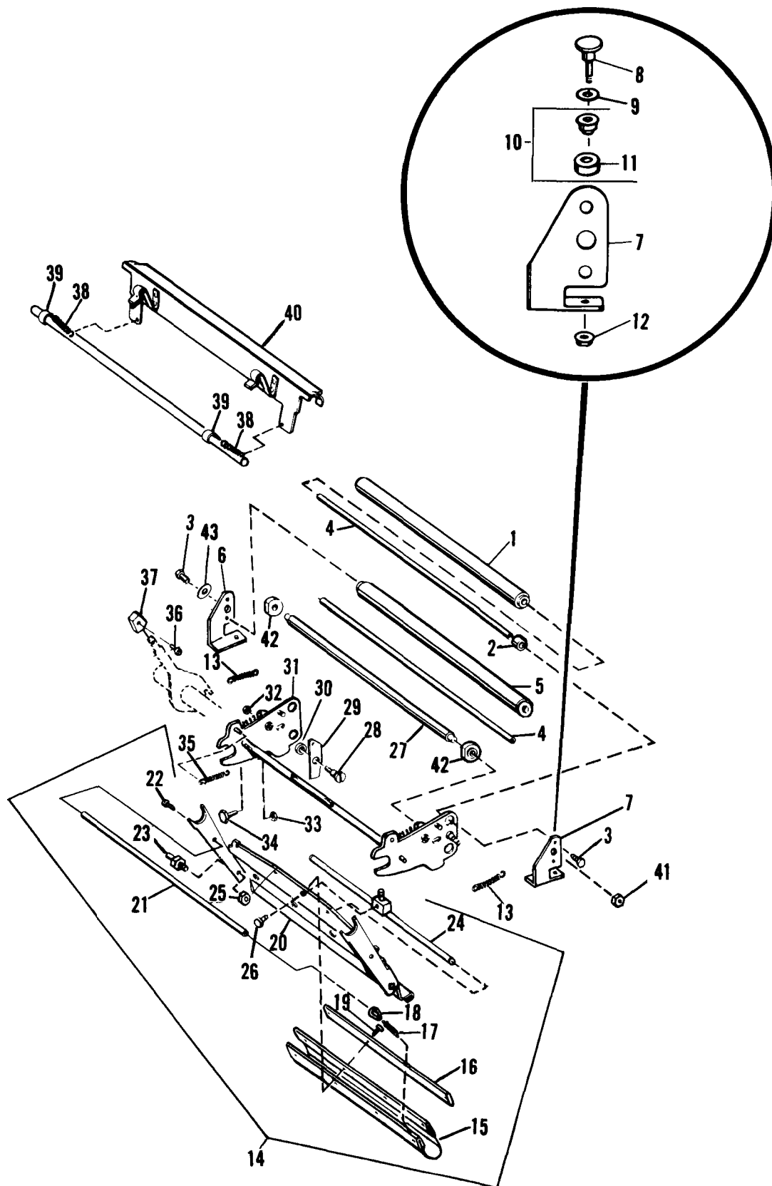
FIGURE 40 - MODEL 9865/9869 Blanket Washer - Part II
