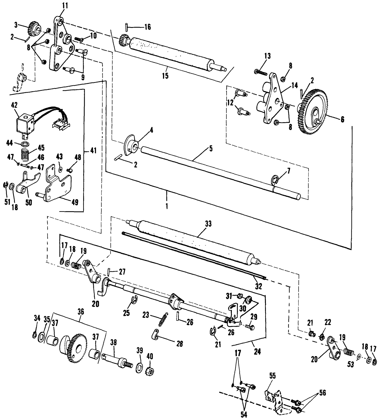
FIGURE 19 - MODEL 9865/9869 Ink Feed Solenoid, Distributor and Ductor Rollers
