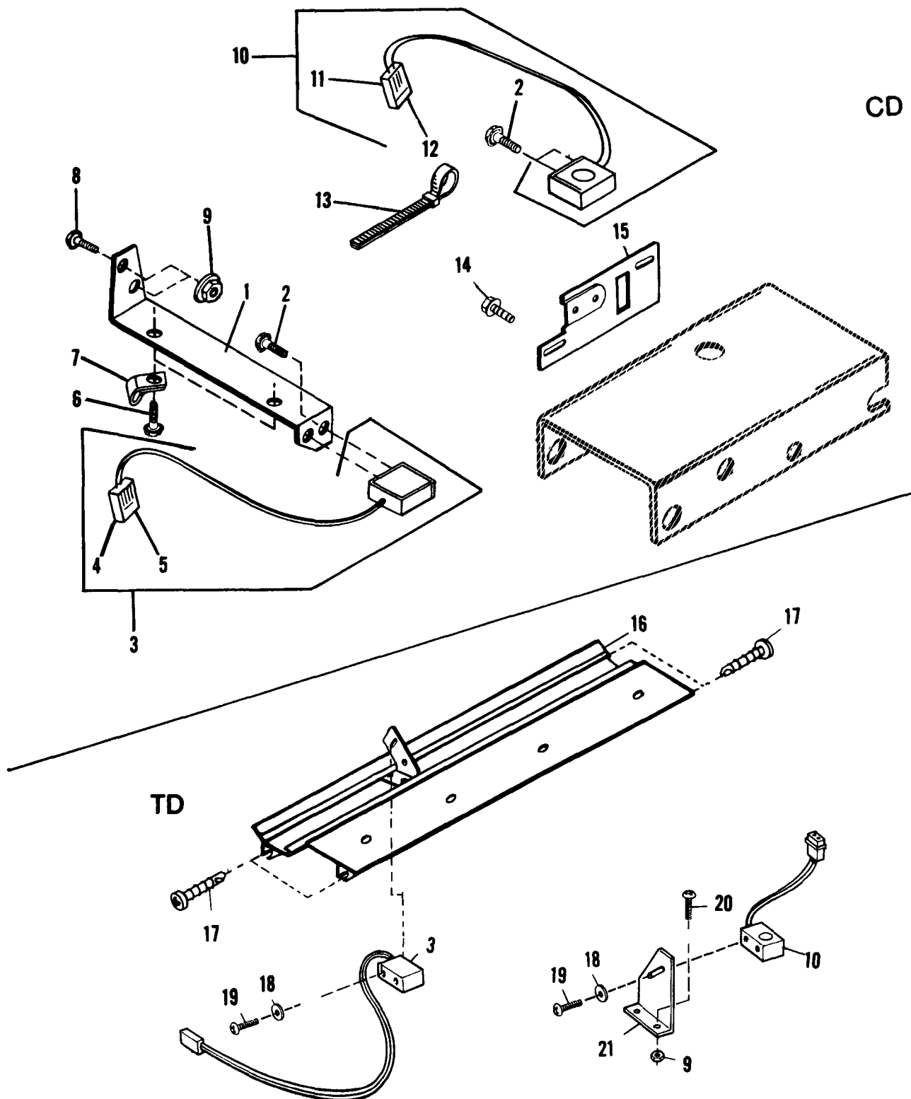
FIGURE 64 - MODEL 9865/9869 Jam Detector Assembly
