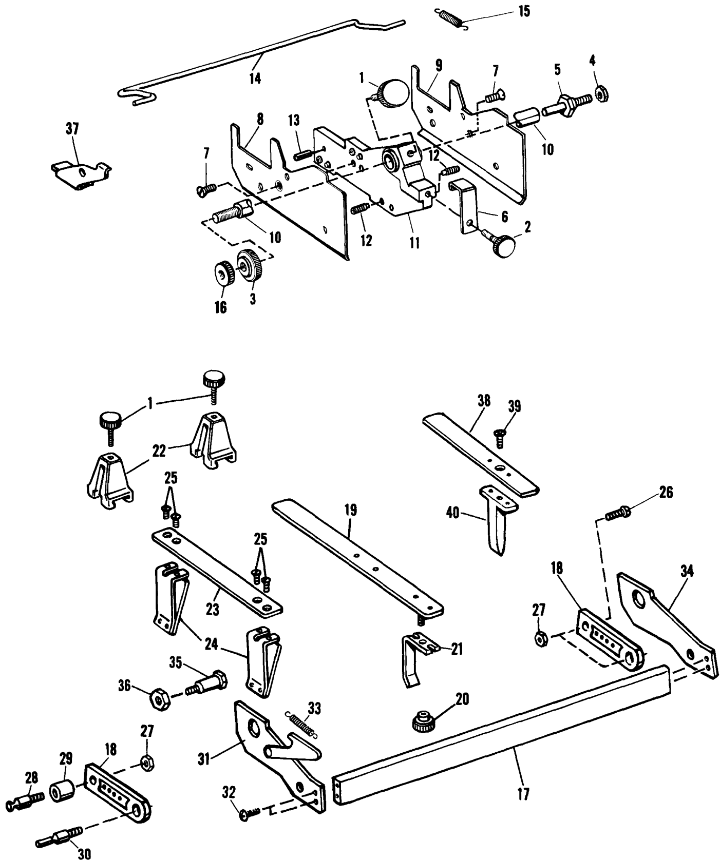
FIGURE 1 - MODEL 9865/9869 Paper Guides and Mounting Bar
