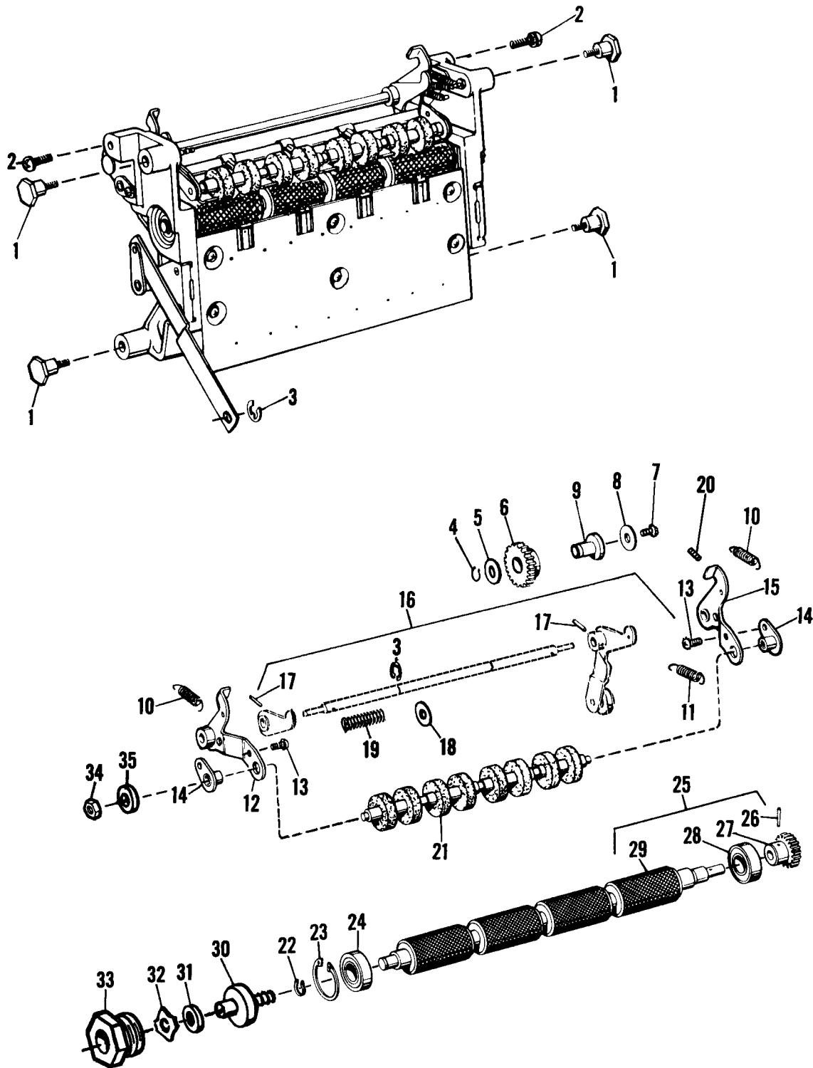
FIGURE 58 - MODEL 9865/9869 Main Tie Bar Assembly - Part I
