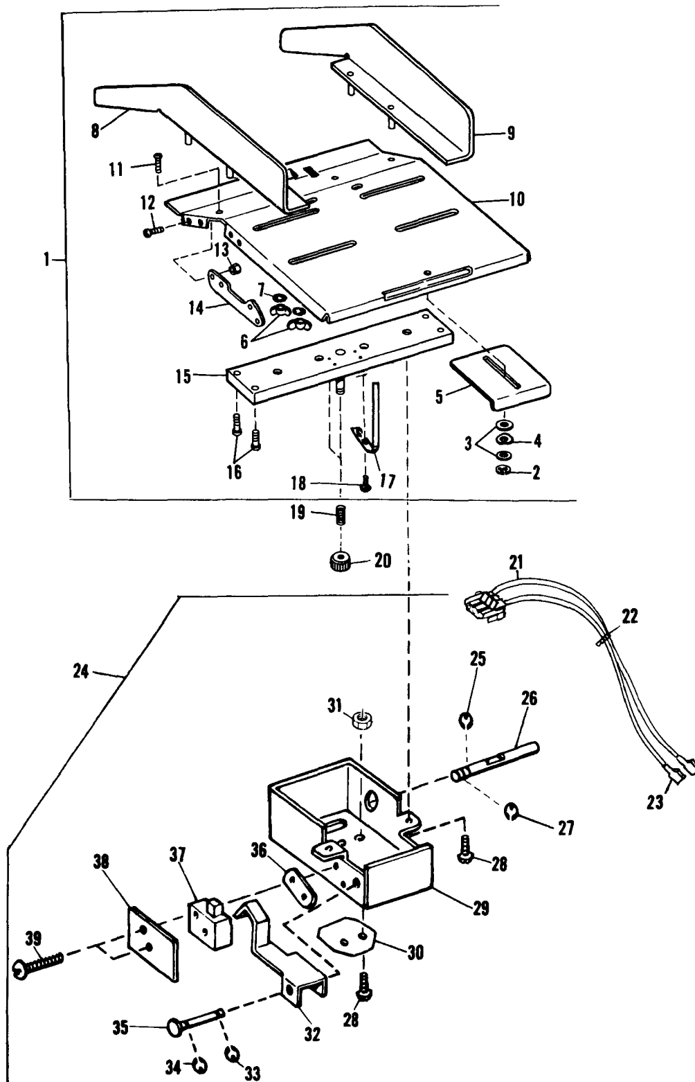
FIGURE 25 - MODEL 9865/9869 Master Feed Table and Switch
