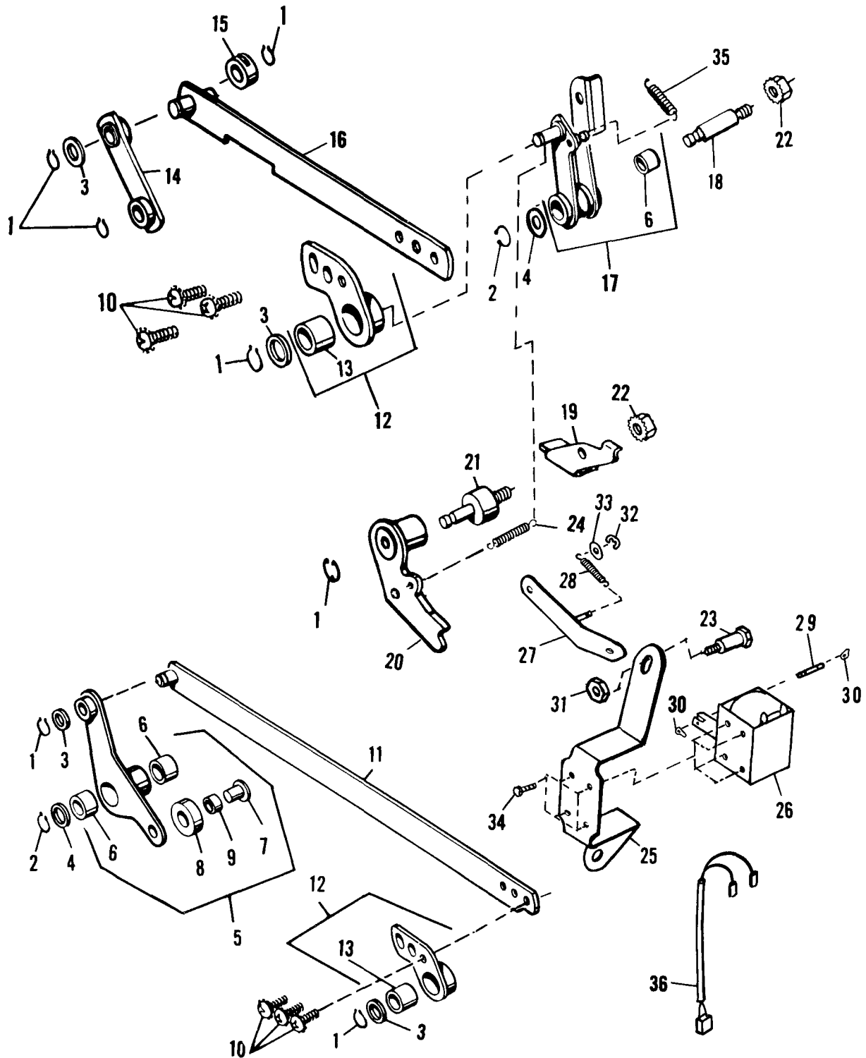
FIGURE 55 - MODEL 9865/9869 Feed Solenoid and Link Assemblies
