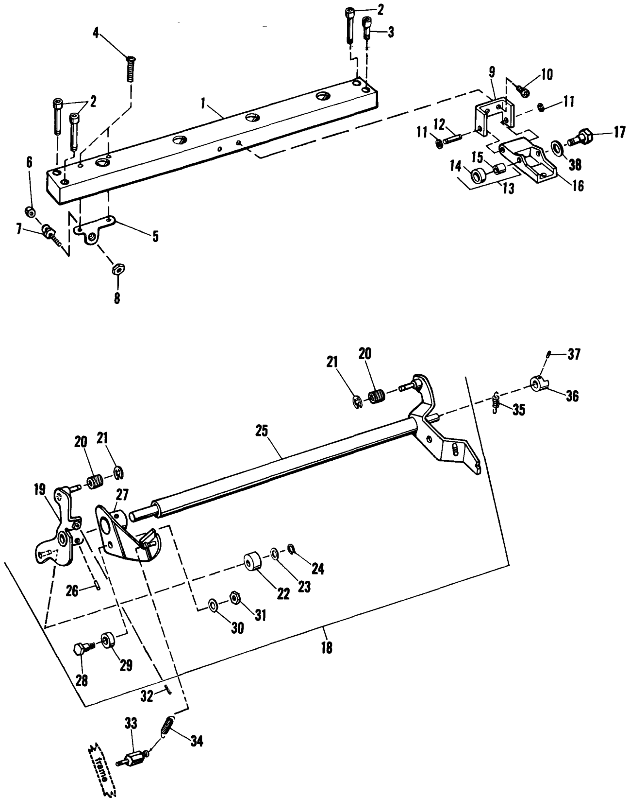
FIGURE 30 - MODEL 9865/9869 Master Forwarding Unit - Part III
