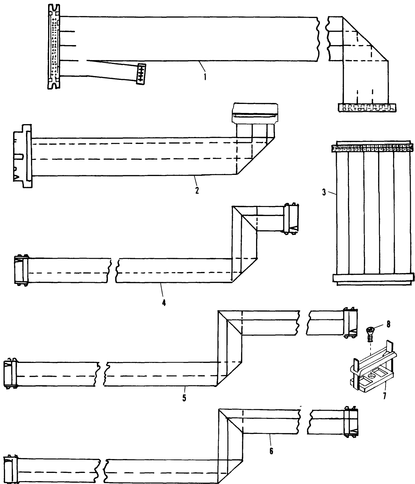
FIGURE 78 - MODEL 9865/9869 Control Box Ribbon Cables
