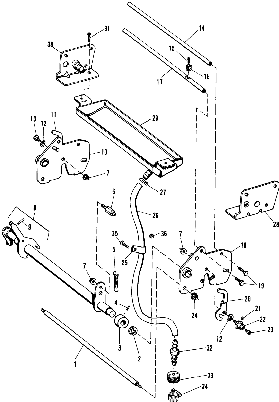
FIGURE 39 - MODEL 9865/9869 Blanket Washer - Part I
