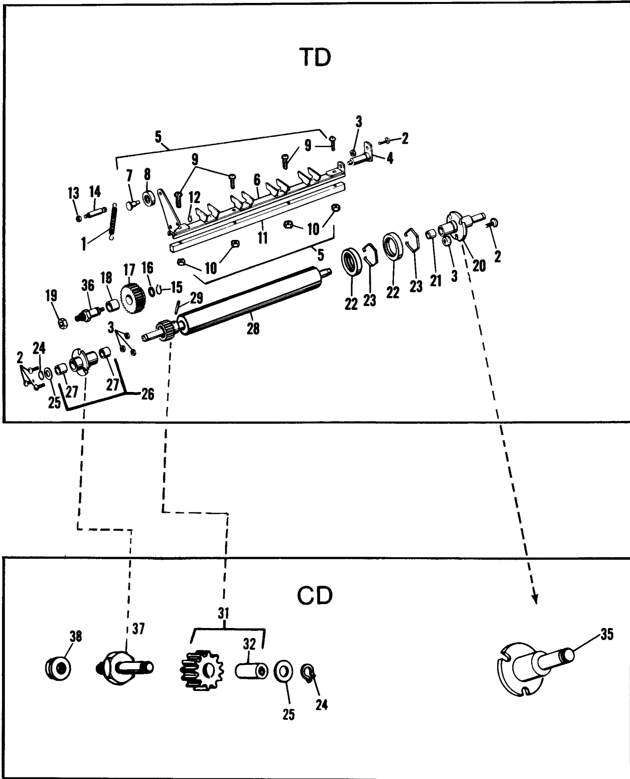
FIGURE 62 - MODEL 9865/9869 Delivery Roller and Stripper Assembly
