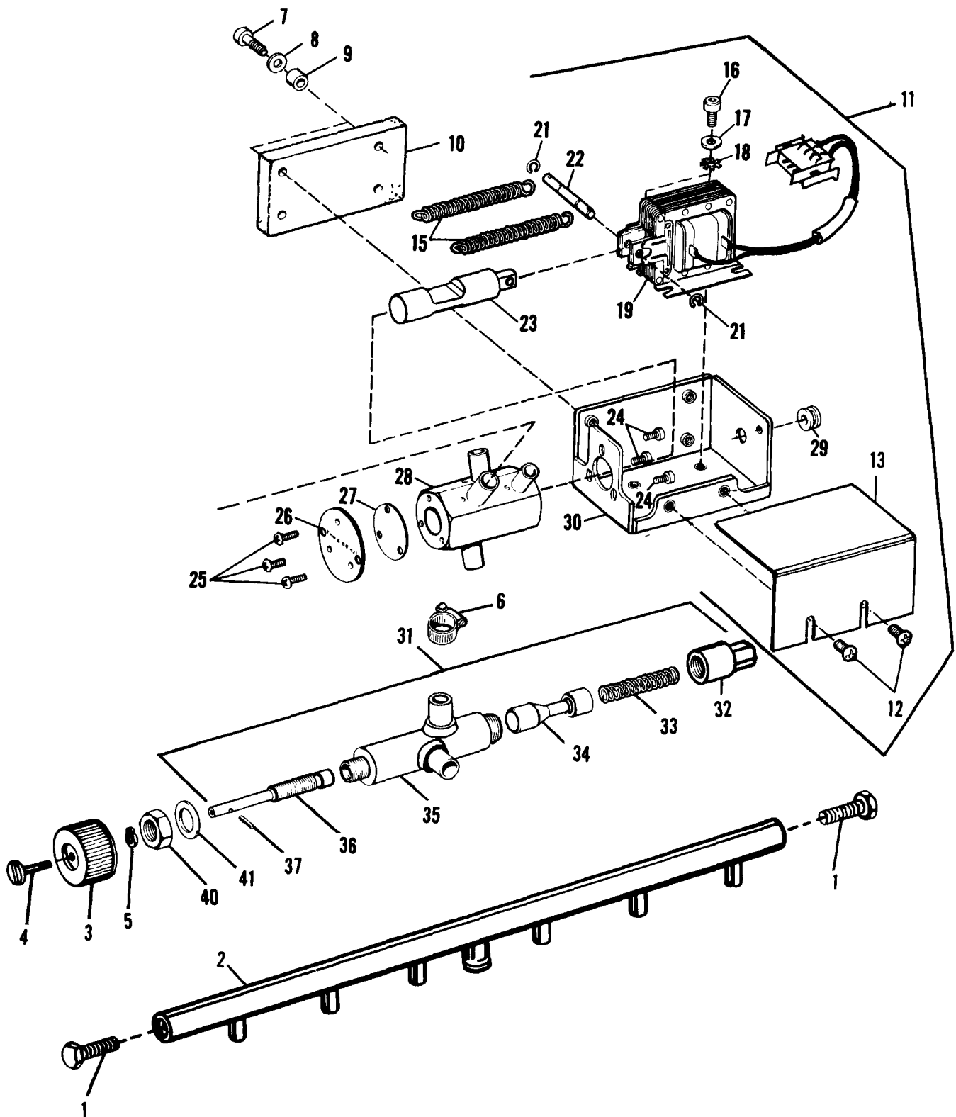
FIGURE 68 - MODEL 9865/9869 Air, Vacuum and Shuttle Valves
