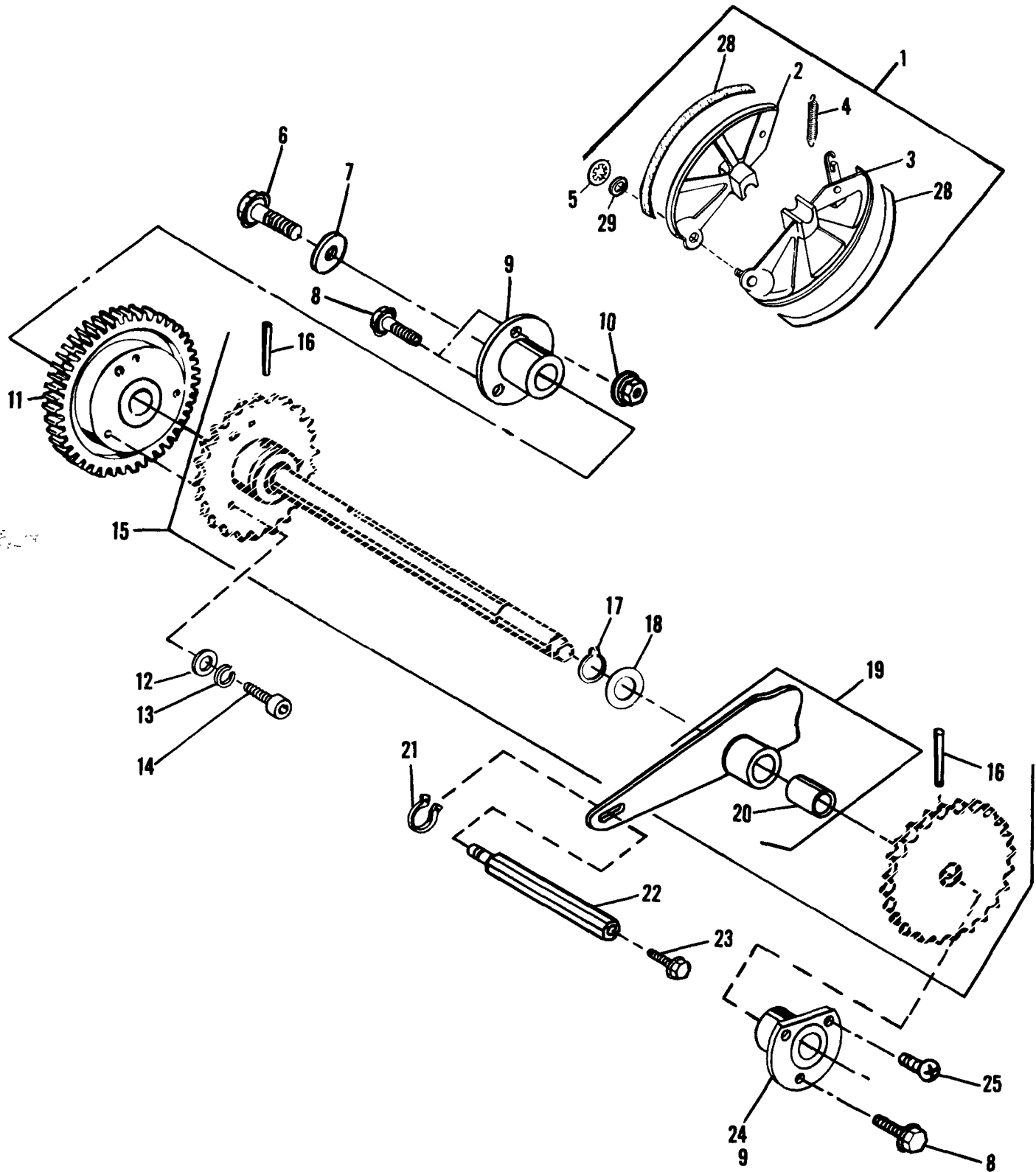
FIGURE 79 - MODEL 9865/9869 Sprocket Shaft and Paper Guides
