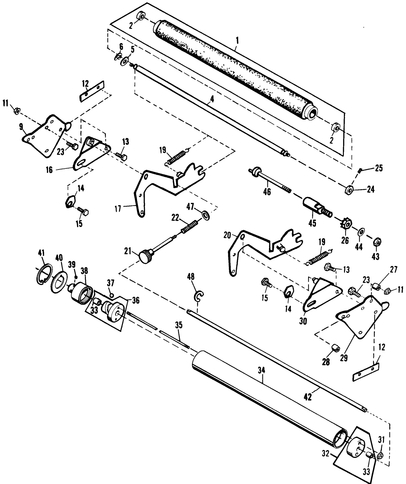
FIGURE 23C - MODEL 9870 Form Roller - Third
