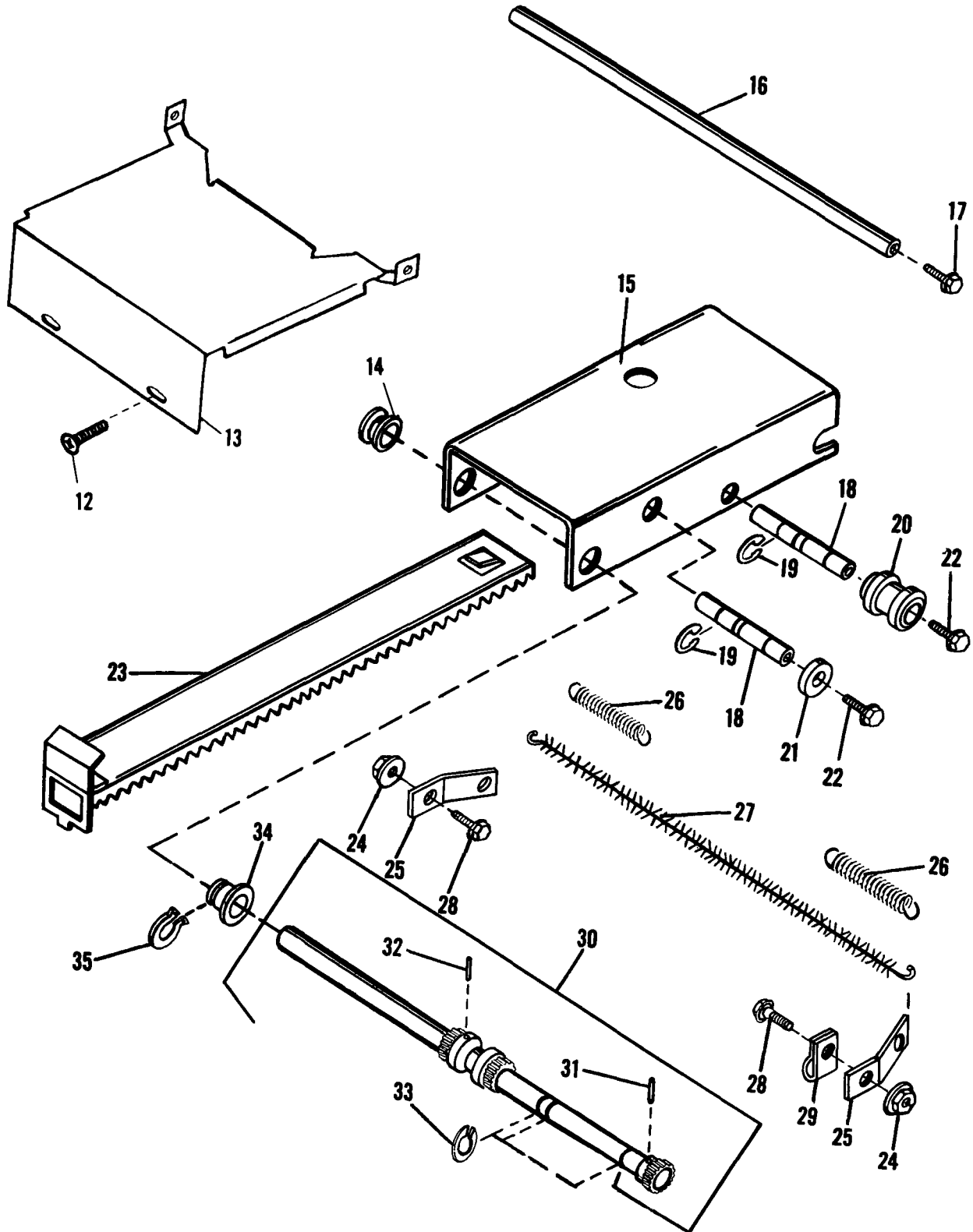
FIGURE 82 - MODEL 9865/9869 Back Jogger Mechanism - Part I
